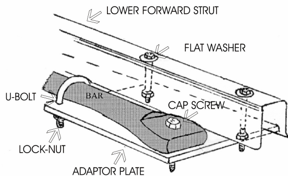
BAR DETAIL MOUNT
